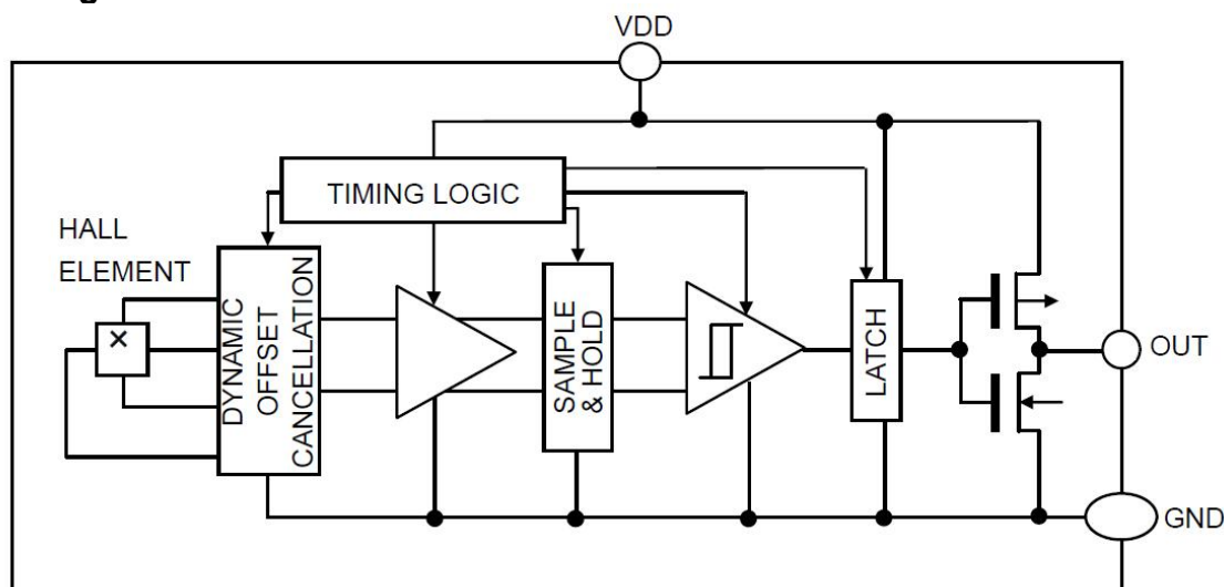
Figure 3, Block Diagram of AS1812B
