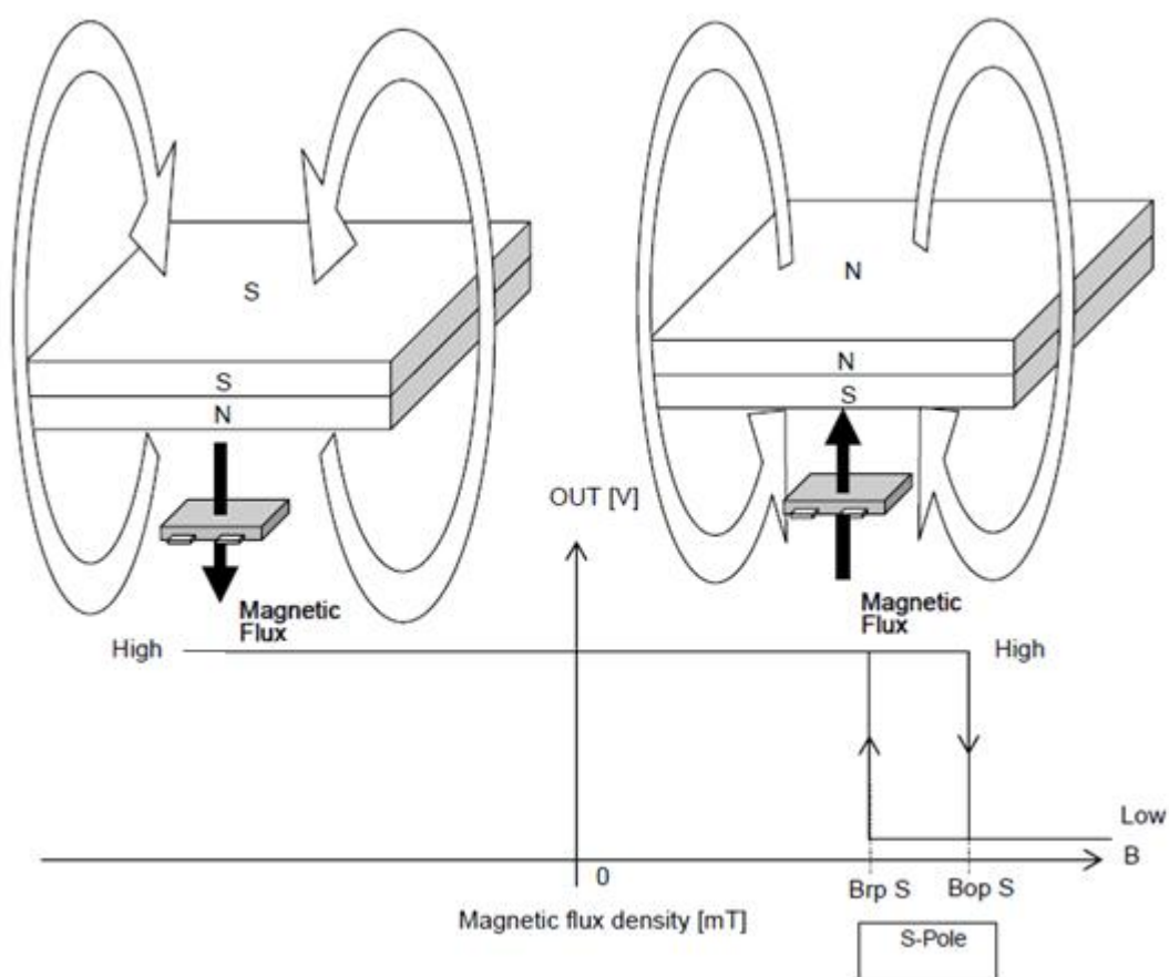
Fig 4, Magnetic Operation Characteristic of AS1812B
