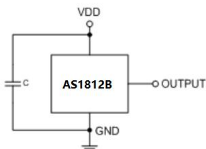
Figure 1, Typical Application Circuit of AS1812B
